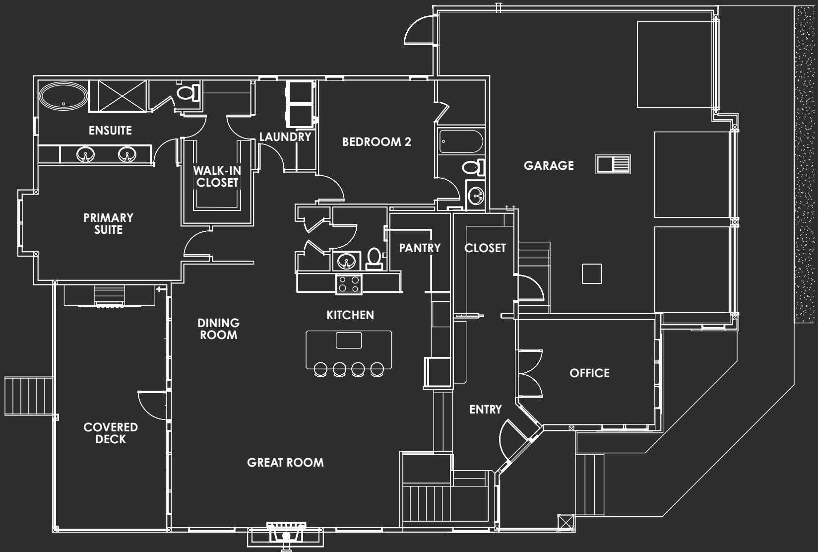
MAIN LEVEL
