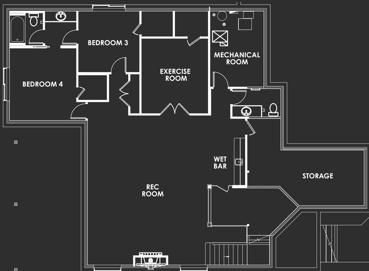
LOWER LEVEL
